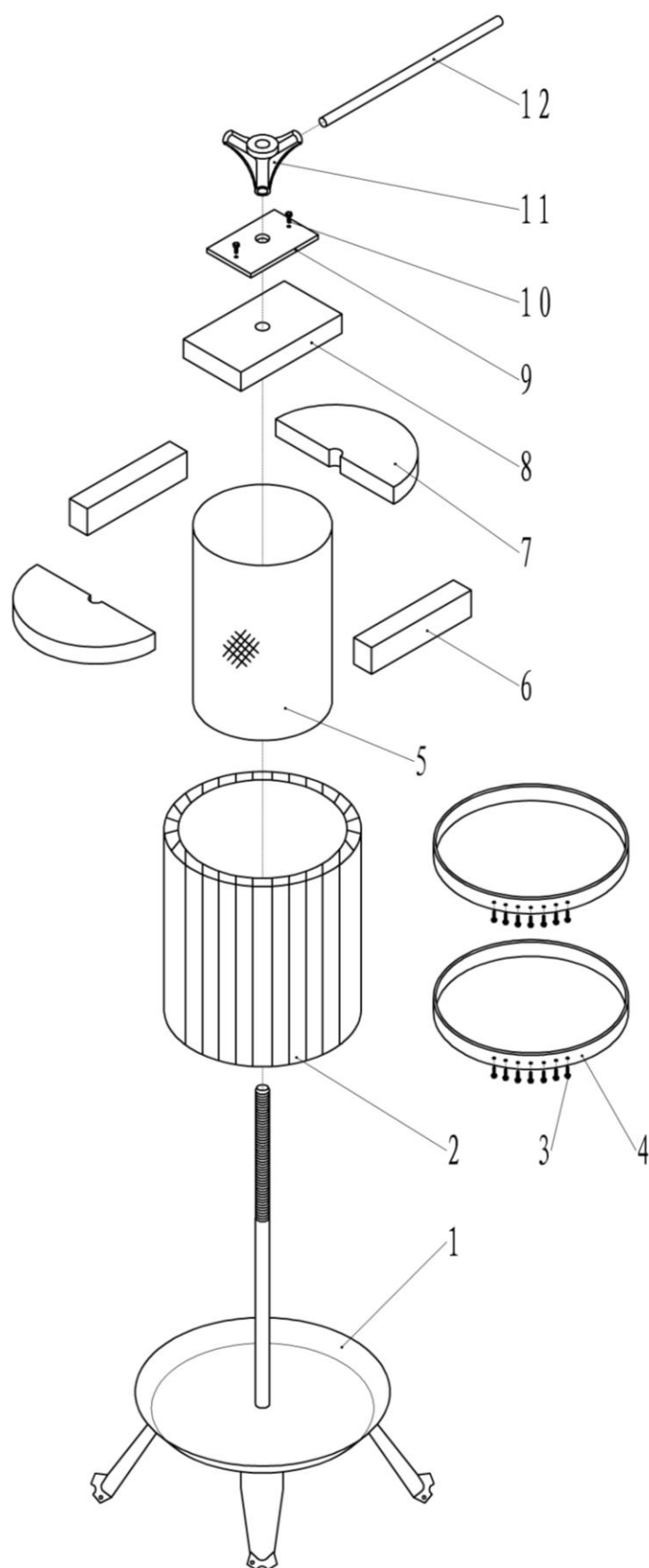
Schema explodata (fig. 3)
