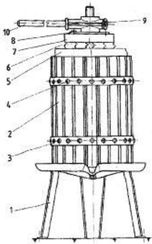
Schema asamblata (fig. 2)
