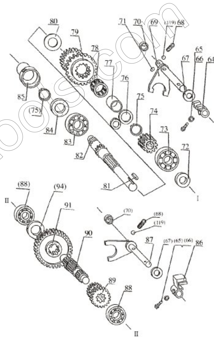
7. Unit of gearbox (6.37.001)
