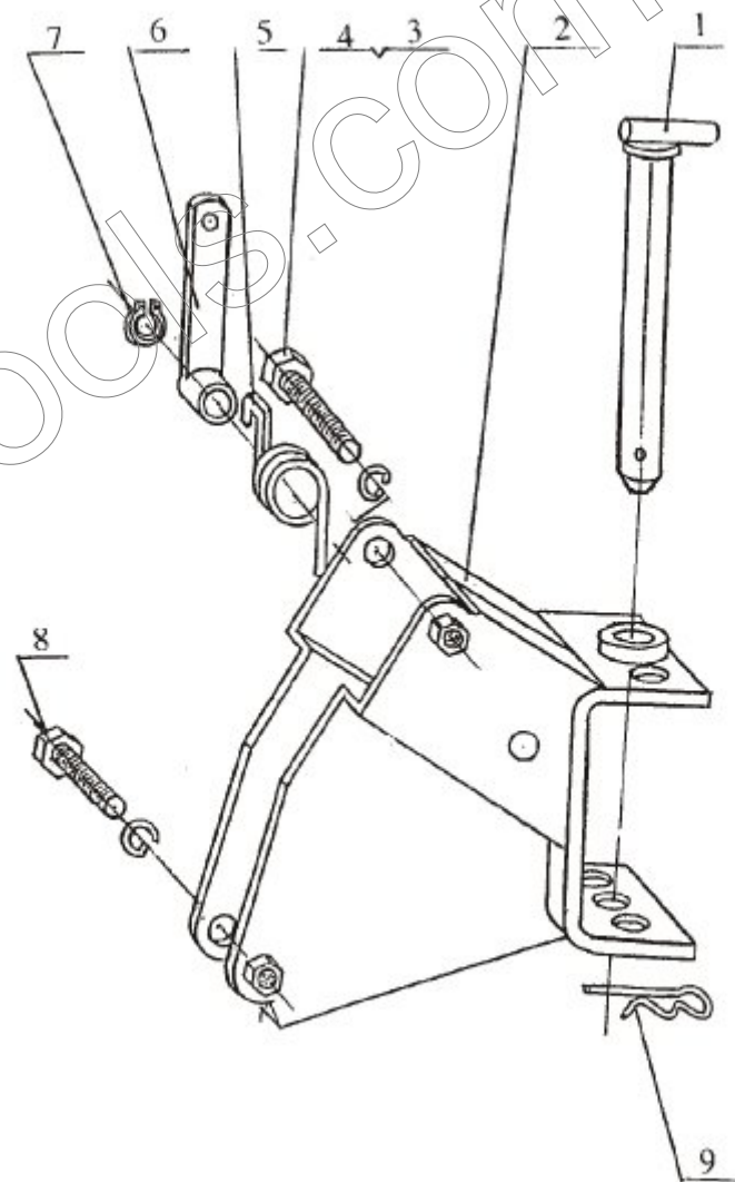
6. Unit of hanging and connecting frame (6.35.001)
