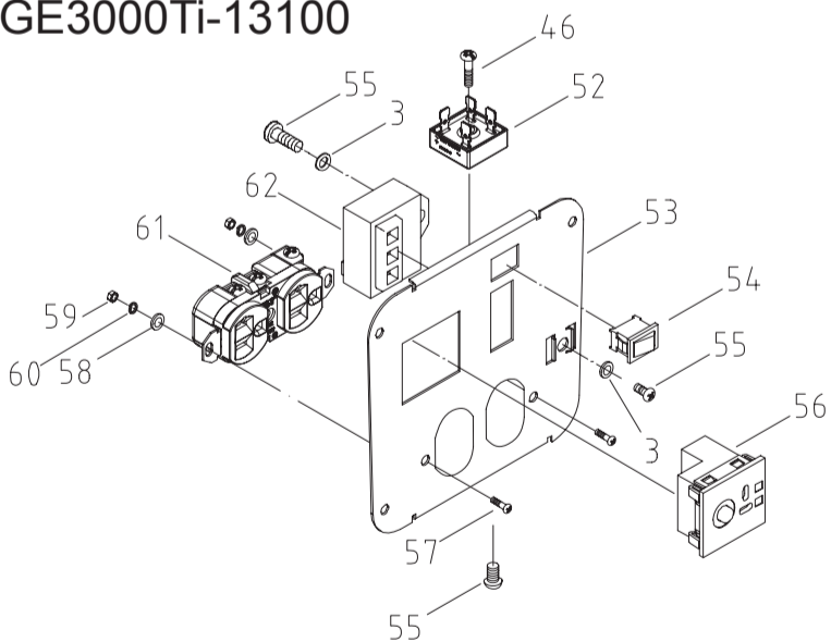
Control Panel Assembly KGE3000Ti-13100
